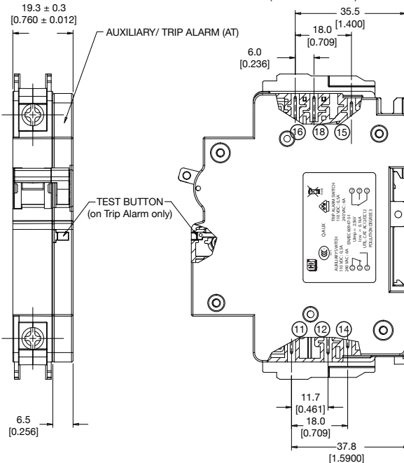
CONNECTING TERMINALS DETAIL (COMMON TO ALL)
